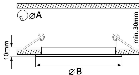
LED PANEL LN18W
